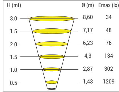
CFT40 24 LED CW 120D 9.6W 24V DC IP44
